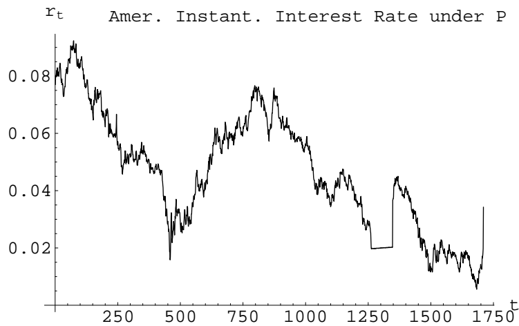
Figure 2: Graphics of r_t in the “real-world” measure.
