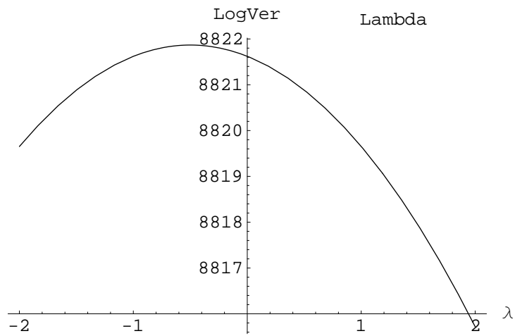
Figure 6: Variation of the log-likelihood changing \lambda^r around the maximum.
