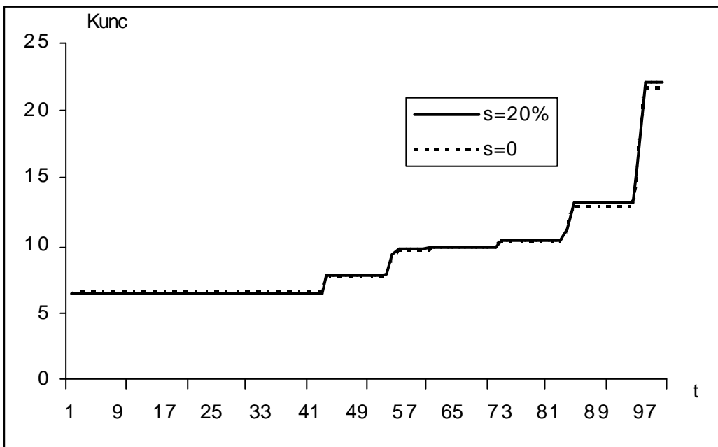
Total capital dynamics with and without tax credit; stochastic case under embodiment
