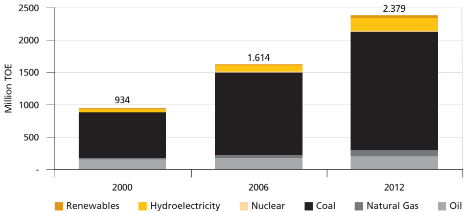
FIGURE 4 Primary energy consumption (In million Toe)
