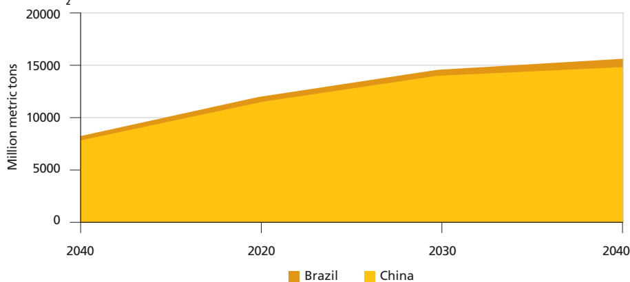
FIGURE 13 CO 2 emissions
