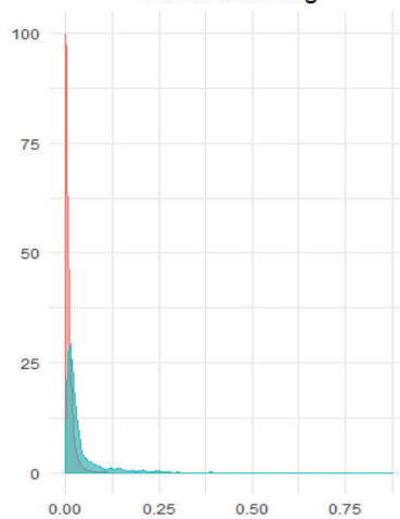
FIGURE A.2 Kernel density, education sample Before matching
